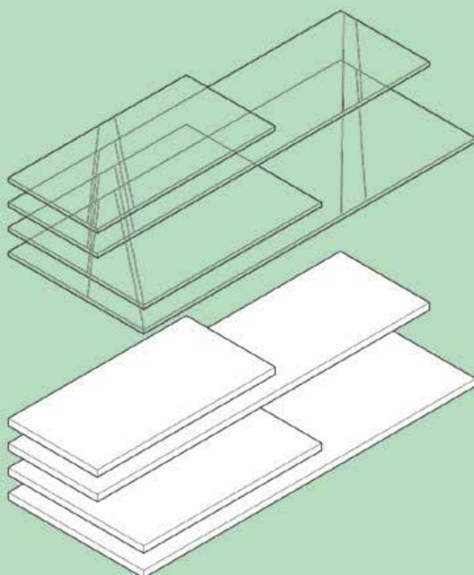
C380/500 Glass Shelf (10mm x 250mm x 500mm) 10kg loading per shelf
